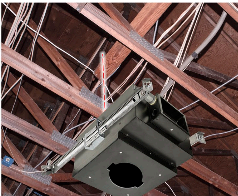
Step 2- Adjustable Mounting Rails anchor housing to ceiling joists with screws
