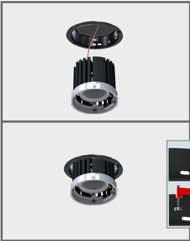
Step E- Finalize electrical wiring/connections. Then slide light assembly into receiver. Step F- Ball plungers(4) on light assembly clicks into 4 slots on receiver.
