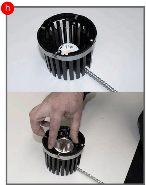
Step H- Install new reflector and optics retainer. Re-install into plaster ceiling.
