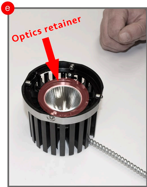
Step E- Locate Optics Retainer (Highlighted in red is the ring that holds the reflector in place).
